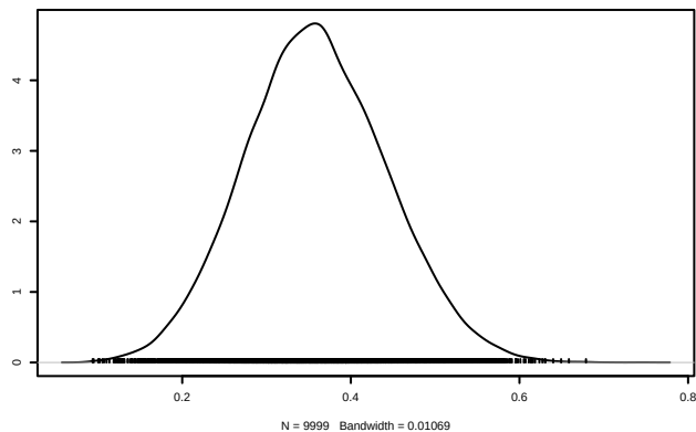
Density of sigma.eps[1]
