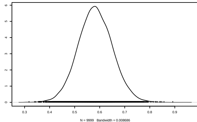
Density of sigma.eps[3]
