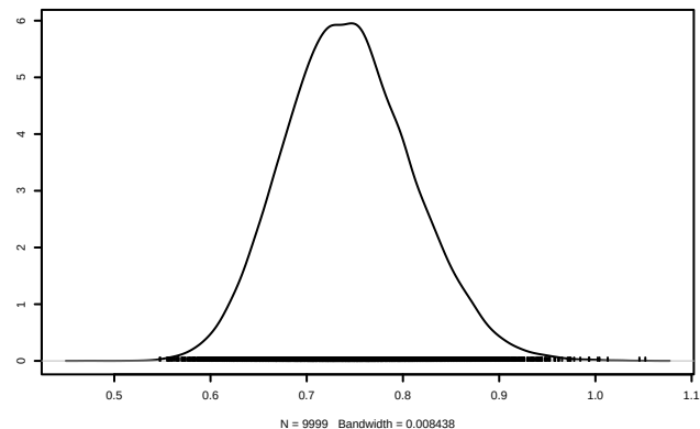
Density of sigma.eta
